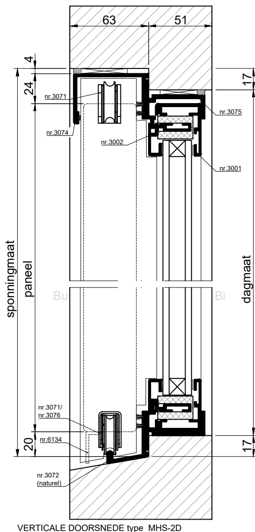
VERTICALE DOORSNEDE type MHS-2D
